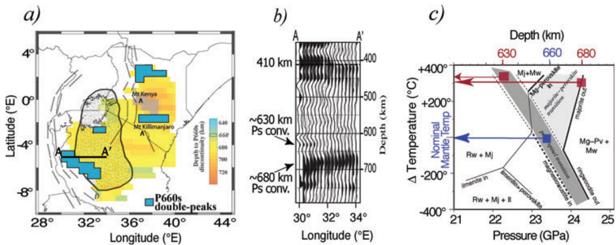
Figure 4. Observations and interpretations of double P_s arrivals near depths of 660 km. (a) Map view showing regions where double arrivals are observed in the high-frequency stacks (blue polygons) overlain on 660-depth map. (b) Cross-section A–A' displaying the double P_s arrivals observed in the high frequency stacks (black; Gaussian = 1.5) overlain on the low-frequency stacks (grey; Gaussian = 0.4). Stacking parameters: a minimum of seven receiver functions per bin from at least three stations, a bin radius of 1.25°, and a bin increment of 0.25°. (c) Phase diagram showing P–T conditions for the majorite → perovskite and post-spinel transitions. Red squares display estimated temperatures at the depths of the observed double arrivals in cross-section A–A' (after Hirose 2002).
