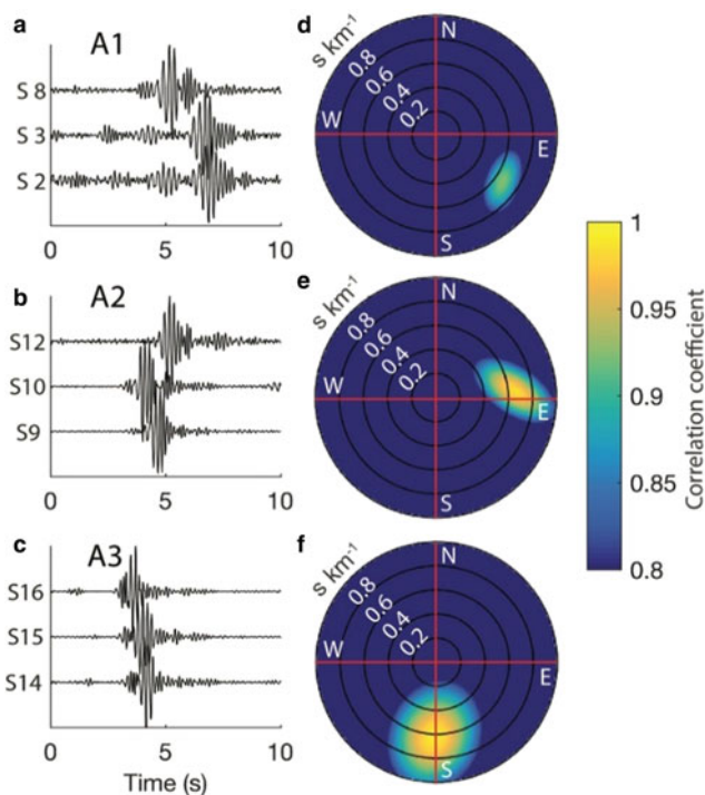
Fig. 5. Example of one seismic event (# 20032 on 2 January 2014 at 2:08 pm, near the end of a rising tide) and the corresponding beamforming result. (a–c) Normalized bandpass filtered waveforms as they arrived at each station in the subarray. (d–f) Probability maps from searching through azimuths for all discrete values of a range of slownesses.
