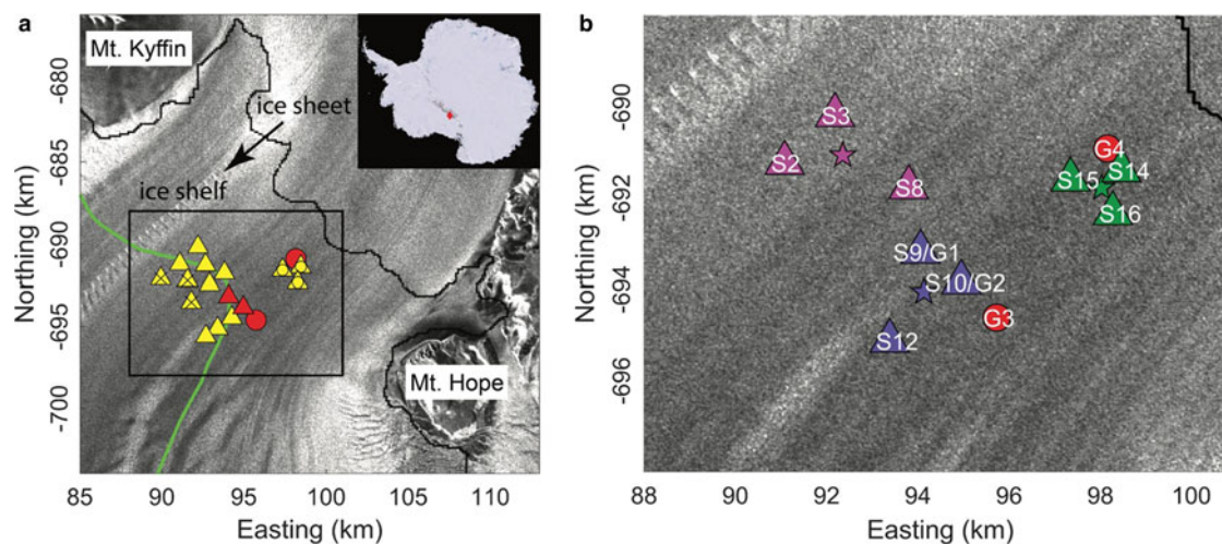
Fig. 1. Study area and station locations, black line is 2004 MOA grounding line (Haran and others, 2005). (a) Yellow triangles denote seismic-station locations and red circles denote GPS station locations. Stations marked with ‘x’ were moved to locations marked with ‘o’ on 30 December. Two GPS stations were located near seismometers and their locations are combined as red triangles. Green line is the freely-floating boundary, or ‘hydrostatic line’ (Bindschadler and others, 2011). (b) Zoom of black box in (a), showing station locations in subarrays; seismometers denoted by ‘S-’; GPS stations denoted by ‘G-’. Array A1 (S2, S3, S8) is marked in pink, A2 (S9, S10, S12) in purple and A3 (S14, S15, S16) in green, with subarray centers marked by stars. Background image is the Radarsat Antarctic Mapping Project (RAMP) mosaic (Jezek and others, 2013).
