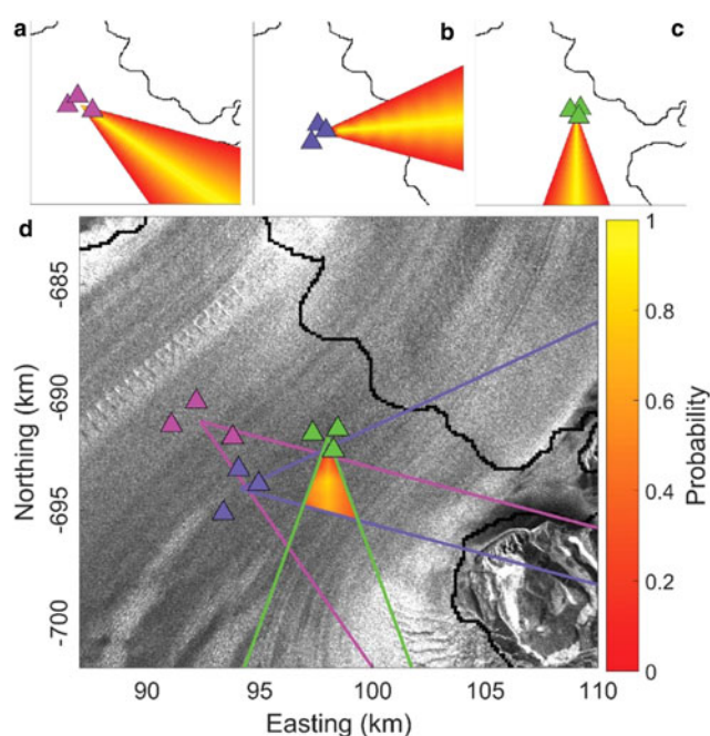
Fig. 6. Well-located event # 20032 shown in Figure 5. Spatial probability distribution wedges for azimuth at arrays (a) A1 (pink), (b) A2 (purple) and (c) A3 (green). (d) Spatial source probability with outlines of wedges that define azimuth estimate \pm 20^\circ for each subarray.
