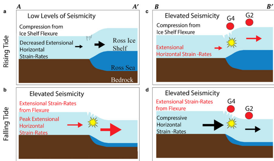
Fig. 8. Schematic of how the two main mechanisms influencing seismicity near grounding zones, vertical ice-shelf flexure and variable horizontal strain rates, vary during the tidal cycle for the two transects shown in Figure 2a and b. The vertical direction is exaggerated for clarity. Processes promoting increased levels of seismicity are in red, those promoting decreased levels of seismicity are in black. Explanation in section ‘Tidal modulation of seismicity’.
