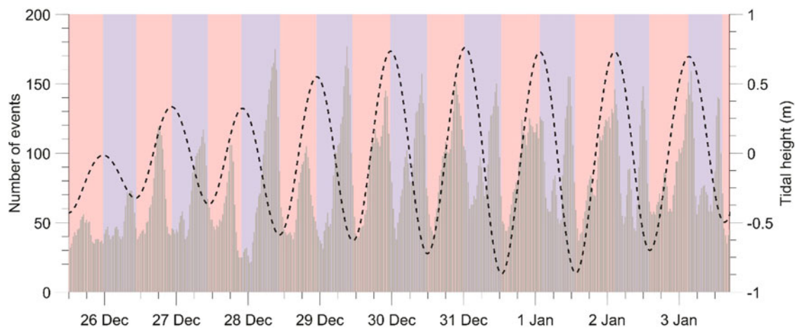
Fig. 4. Temporal pattern of seismicity, displayed in 30 min bins using a 3 h moving average. Rising tide is highlighted in red, falling tide in blue. Tidal height is estimated from the vertical motion of station G2.
