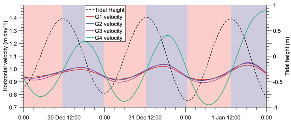
Fig. 3. Tidal variation in horizontal velocity measured by GPS stations. Tidal height is estimated from the vertical motion of station G2. Stations move slower during rising tides (shaded in red), and faster during falling tides (shaded in blue).
