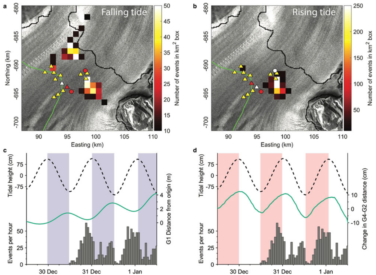
Fig. 7. Locations of events occurring during (a) falling tide and (b) rising tide. Boxes with less than ten events are not pictured. For (c) and (d) histograms of well-located events in grey (no well-located events on 30 December as A3 was not in place), black dashed line is tidal height (from G2), falling tide shaded in blue and rising tide shaded in red. (c) Line in green is the change in location of station G1, the white triangle in (a). The speed of G1 is tidally modulated, and the station moves slowly downstream, \sim 4 m over the 4 d pictured. (d) Line in green is horizontal distance between stations G2 and G4, the white triangle and circle respectively in (b).
