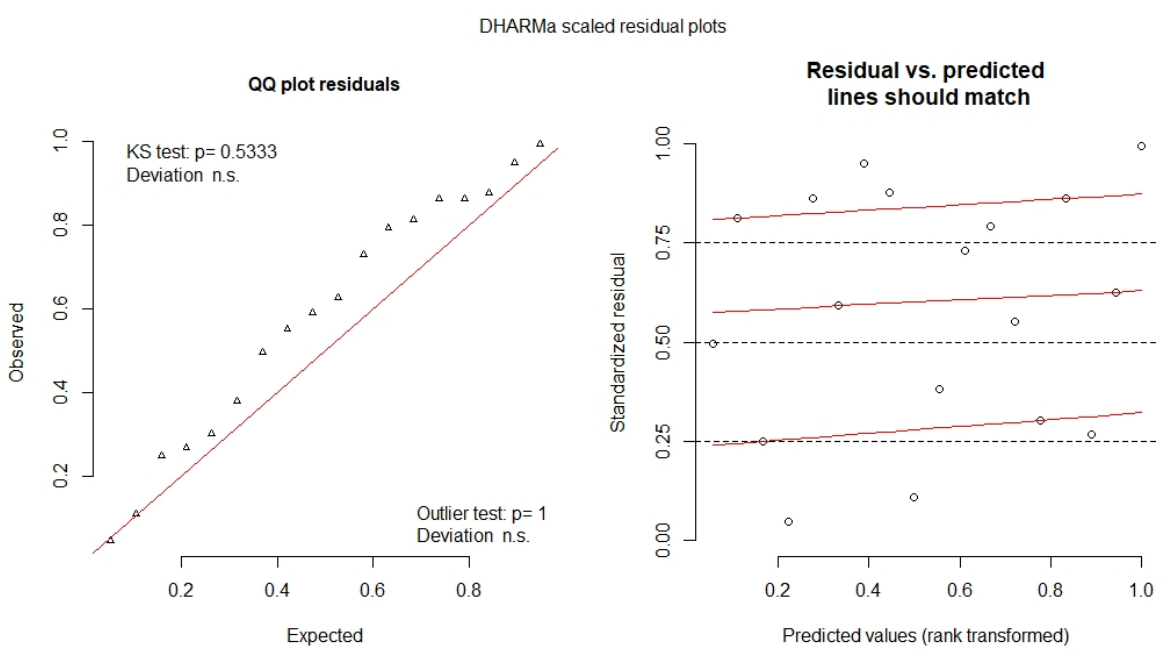
Figure 4. Improved DHARMA scaled residual plots
