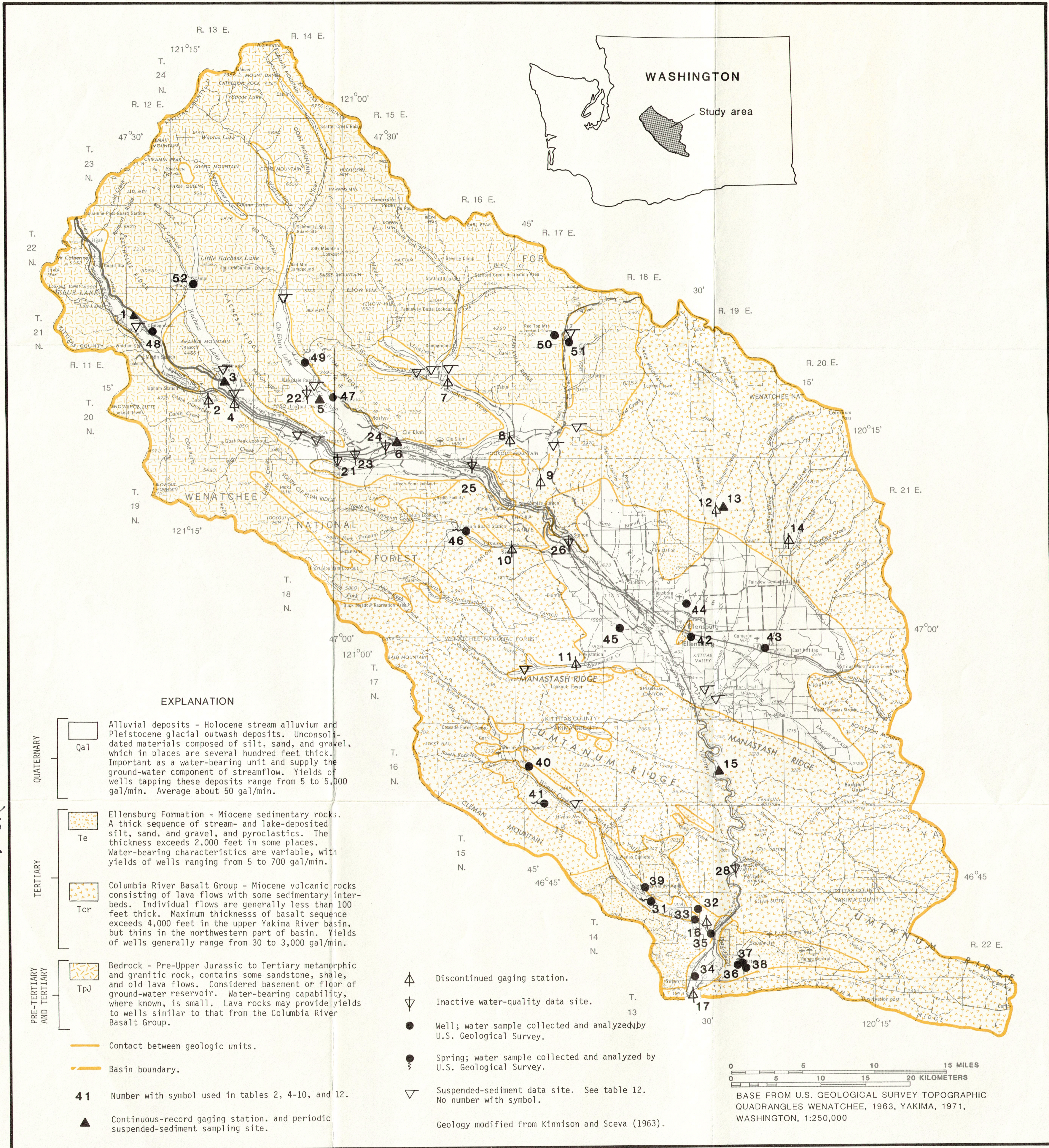
PLATE 1.--Generalized geology and selected data-collection sites in the upper Yakima River basin.
